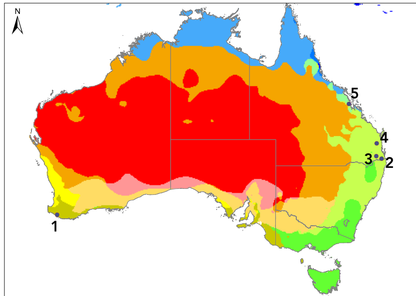
Figure 2. Map of the Australian example catchments for the modeling experiment of flux mapping. The color scheme is based on the Köppen-Geiger climate classification by Peel et al. (2007).
