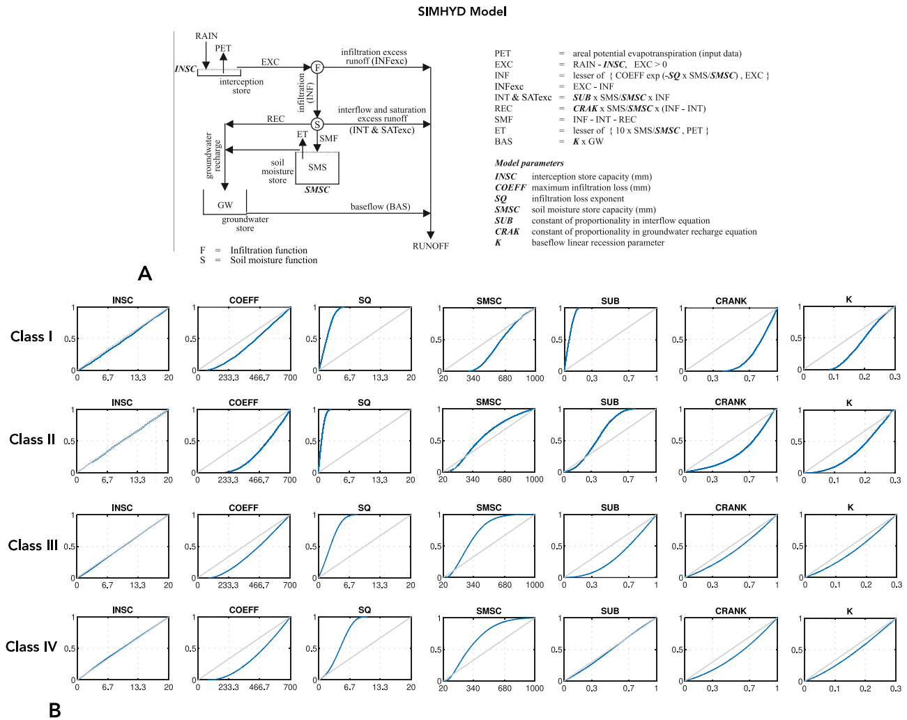
Figure 5. (a) Schematic illustration of the SIMHYD model structure together with the description of the model's internal fluxes and parameters (derived from Peel et al., 2000). (b) Marginal (cumulative) distribution of model parameters (gray is the prior, and blue is the posterior distributions) corresponding to the Classes I–IV flux maps (excluding the extreme case of Class IV) in section 4, for the relaxed threshold ( 0.85 \times SCE\text{-}NSE ).
