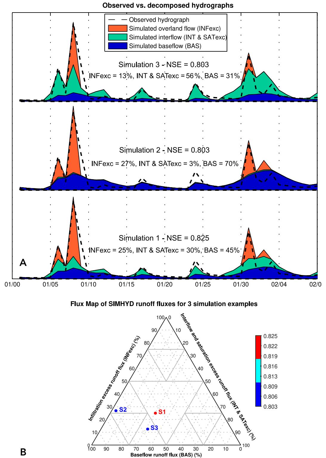
Figure 1. (a) Three simulations (S1–S3) of an observed hydrograph through different combinations of runoff generating mechanisms (volumetric contribution to the total simulated runoff) summarized on a flux map (b), color coded based on the simulation performance (NSE value). The triangle (B) represents the plausible flux space for a model with three runoff fluxes. NSE = Nash-Sutcliffe model efficiency.
