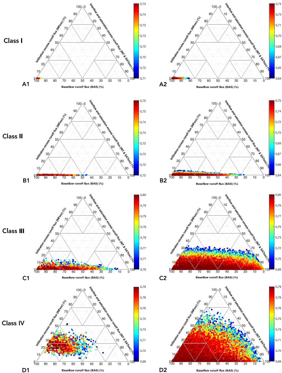
Figure 3. This figure represents how different model internal behavior, represented on flux maps, can emerge within a certain range of model performance. Flux maps for four different Australian catchments (catchments 1–4 on Table 1) for two different thresholding; each row presents a different catchment with strict threshold on the first column and relaxed threshold on the second column. Color bar represents the model performance in terms of Nash-Sutcliffe model efficiency value. (a) Class I flux maps for strict threshold ( 0.95 \times \text{SCE-NSE} = 0.71 \leq \text{Ensemble-NSE} = 0.75 \leq \text{SCE-NSE} = 0.75 ) with 252 equifinal simulations (a1) and relaxed threshold ( 0.85 \times \text{SCE-NSE} = 0.64 \leq \text{Ensemble-NSE} \leq \text{SCE-NSE} ) with 3,036 equifinal simulations (a2). (b) Class II flux maps for strict threshold ( 0.95 \times \text{SCE-NSE} = 0.71 \leq \text{Ensemble-NSE} = 0.75 \leq \text{SCE-NSE} = 0.75 ) with 592 equifinal simulations (b1) and relaxed threshold ( 0.85 \times \text{SCE-NSE} = 0.64 \leq \text{Ensemble-NSE} \leq \text{SCE-NSE} ) with 8,476 equifinal simulations (b2). (c) Class III flux maps for strict threshold ( 0.95 \times \text{SCE-NSE} = 0.74 \leq \text{Ensemble-NSE} = 0.78 \leq \text{SCE-NSE} = 0.78 ) with 3,644 equifinal simulations (c1) and relaxed threshold ( 0.85 \times \text{SCE-NSE} = 0.66 \leq \text{Ensemble-NSE} \leq \text{SCE-NSE} ) with 47,702 equifinal simulations (c2). (d) Class IV flux maps for strict threshold ( 0.95 \times \text{SCE-NSE} = 0.71 \leq \text{Ensemble-NSE} = 0.75 \leq \text{SCE-NSE} = 0.75 ) with 1,270 equifinal simulations (d1) and relaxed threshold ( 0.85 \times \text{SCE-NSE} = 0.64 \leq \text{Ensemble-NSE} \leq \text{SCE-NSE} ) with 65,126 equifinal simulations (d2). Catchment summaries are presented in Table 1.
