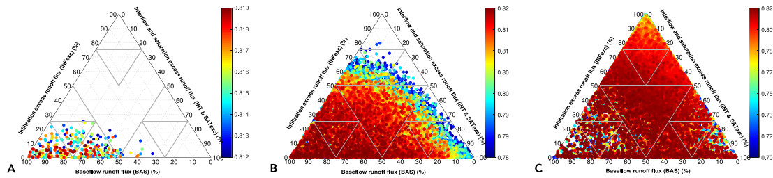
Figure 4. Class IV flux maps for very strict threshold ( 0.99 \times \text{SCE-NSE} = 0.80 \leq \text{Ensemble-NSE} = 0.80 \leq \text{SCE-NSE} ) with 287 equifinal simulations (a), strict threshold ( 0.95 \times \text{SCE-NSE} = 0.77 \leq \text{Ensemble-NSE} \leq \text{SCE-NSE} ) with 69,090 equifinal simulations (b), and relaxed threshold ( 0.85 \times \text{SCE-NSE} = 0.69 \leq \text{Ensemble-NSE} \leq \text{SCE-NSE} ) with 49,591 equifinal simulations only from 10^5 simulations (c). Catchment summaries are presented in Table 1.
